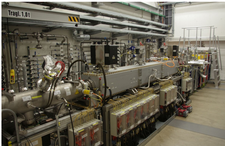
Radiofrequenz-Linac
