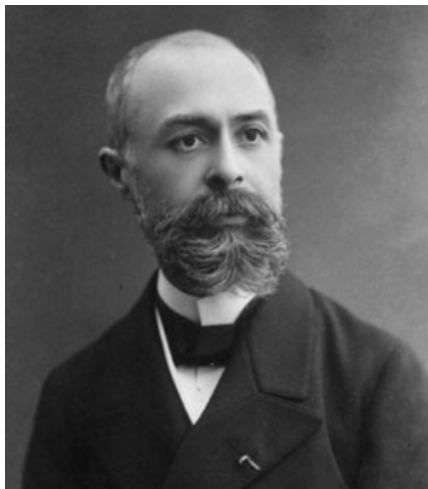
Henri Becquerel
